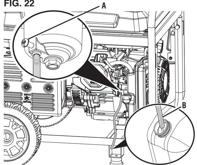
A - Drain screw B - Drain hose
