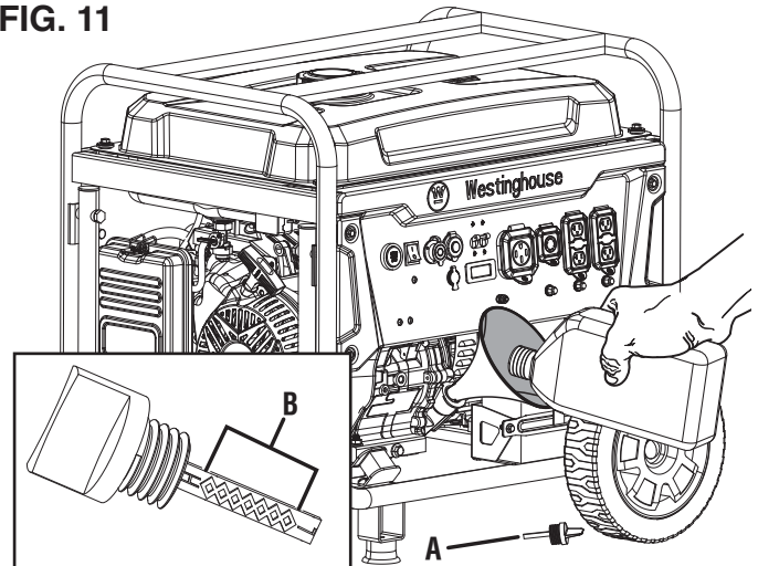
A - Oil dipstick B - Safe operating range
