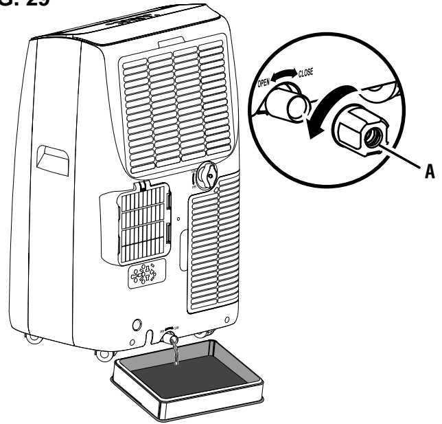
A - Lower Drain Plug
