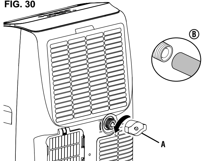
A - Upper Drain Plug B - Connect Drain Hose
